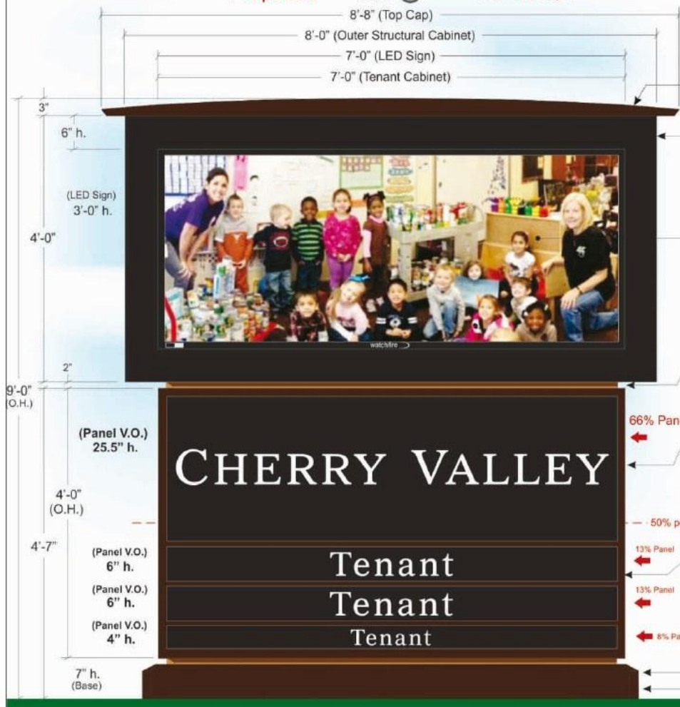
Sign Monument Elevation
